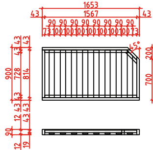
Balustrade for stairs
