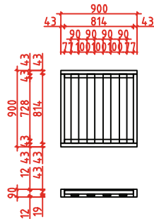
Balustrade for stairs
