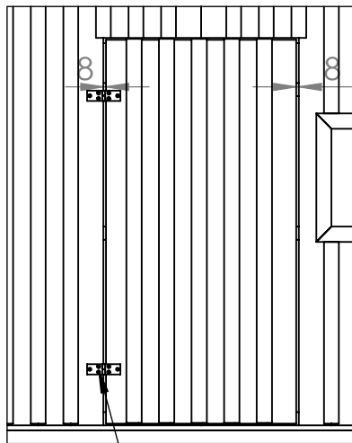
Hinge+35mm screws
